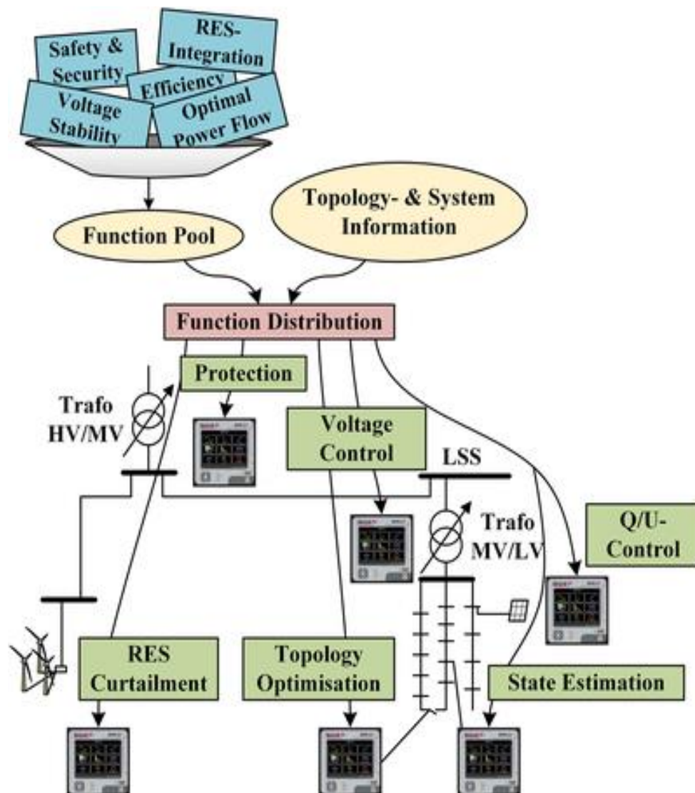
Figure 2: Concept of the proposed smart grid automation system
