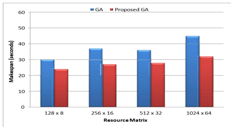
Figure 1 Comparison of Makespan (turnaround time)
