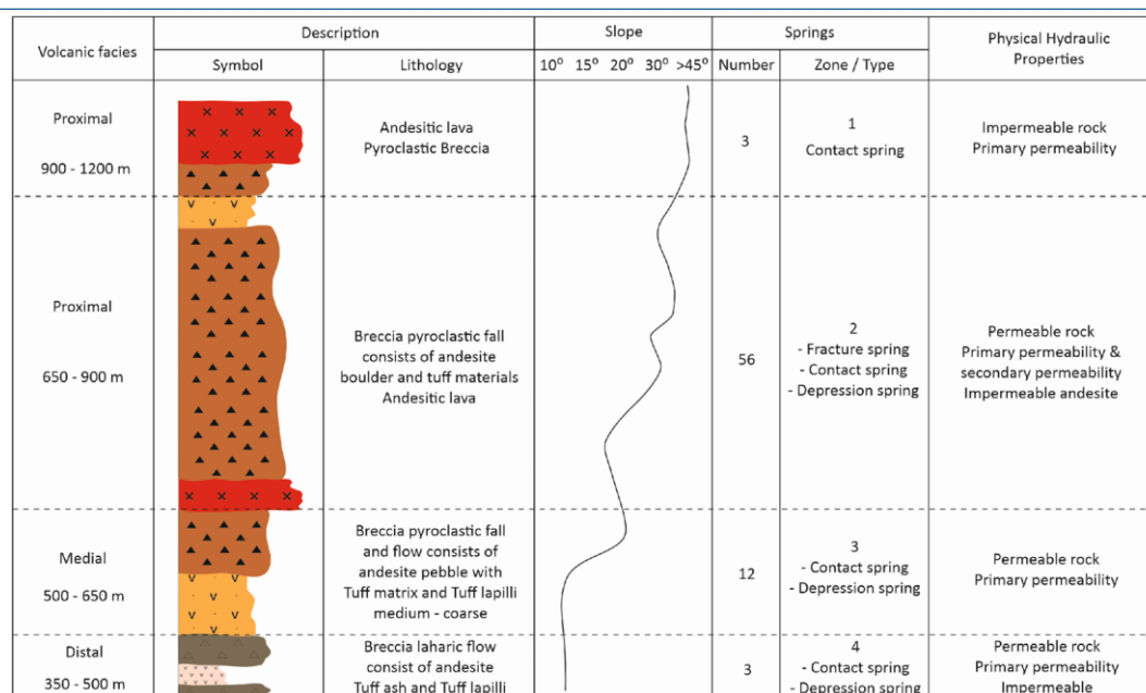
Figure 6. Correlation of lithological facies, morphology and distribution of springs and hydrogeological systems on the slopes of Mount Salak and Mount Pangrango.
