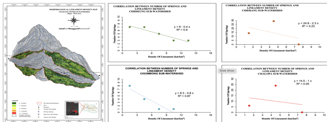
Figure 12. Correlation analysis of lineament/structure density on spring hydrogeological systems
