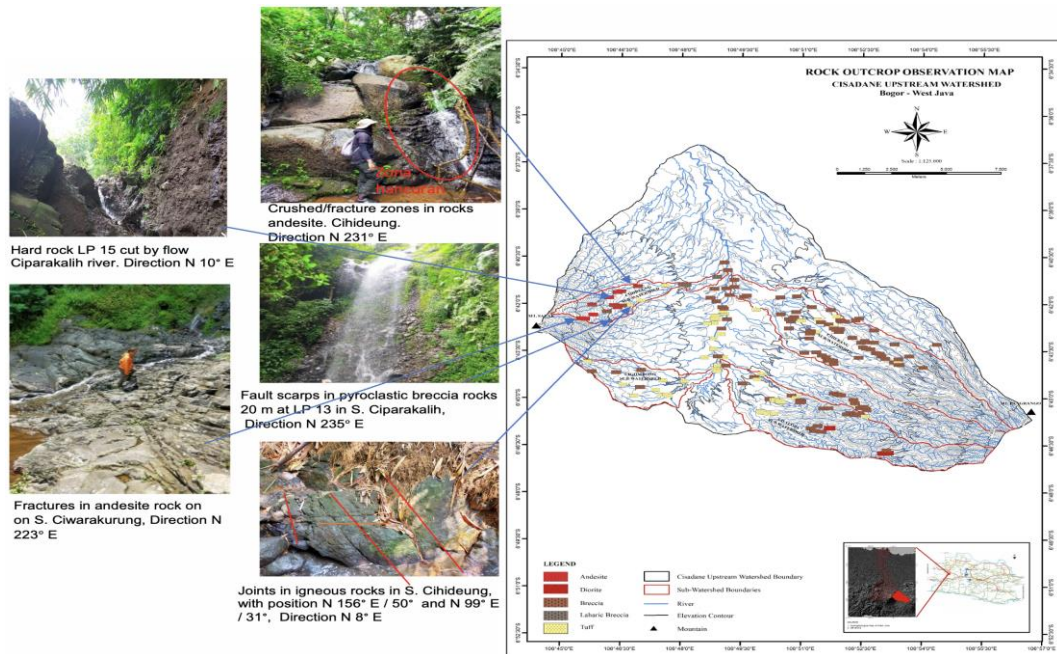
Figure 11. Field observations on the slopes of Mount Salak and Mount Pangrango
