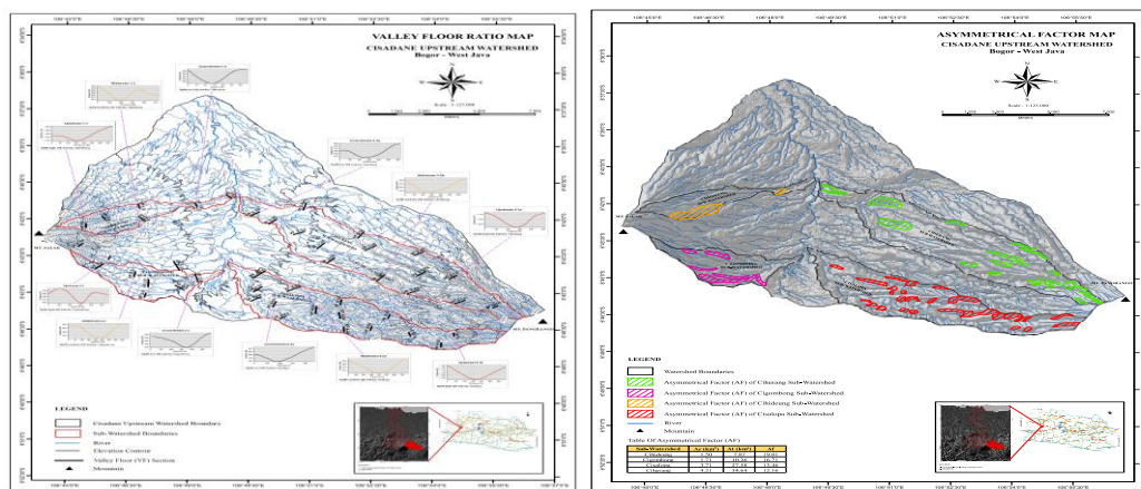
Figure 10. Morphotectonic analysis, Sinuosity Mountain Front SME, Vally Floor VF and Asymmetry Factor AF
