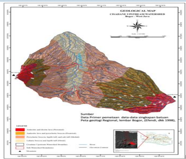
Figure 5. Geological map of Cisadane upstream watershed
