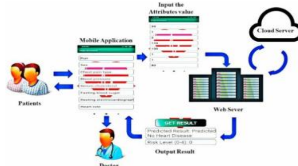
Fig2: - Architecture Diagram
