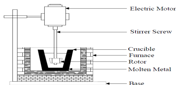
Fig. 1 Stir casting process to fabricate MMC [1]
