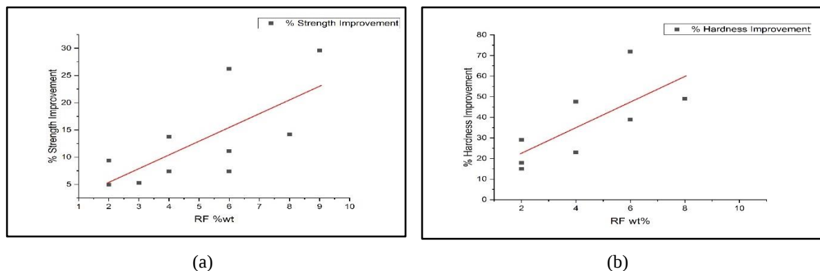
Figure 4: % Strength and Hardness improvement with varying the SiC wt%
