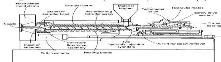
Figure 1. Schematic diagram of molding machine
