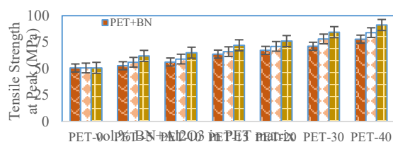
Fig. 3.4, Tensile strength at Peak of PET+BN, PET+ \text{Al}_2\text{O}_3 and PET-BN+ \text{Al}_2\text{O}_3 Composite
