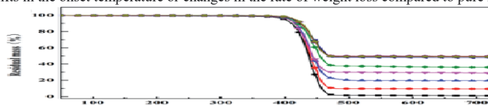
Fig. 3.8, Thermo Gravimetric analysis (TGA) of PET-BN+ \text{Al}_2\text{O}_3 Composite
