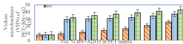
Fig. 3.2, Microhardness of PET+BN, PET+ Al 2 O 3 and PET-BN+ Al 2 O 3 Composite
