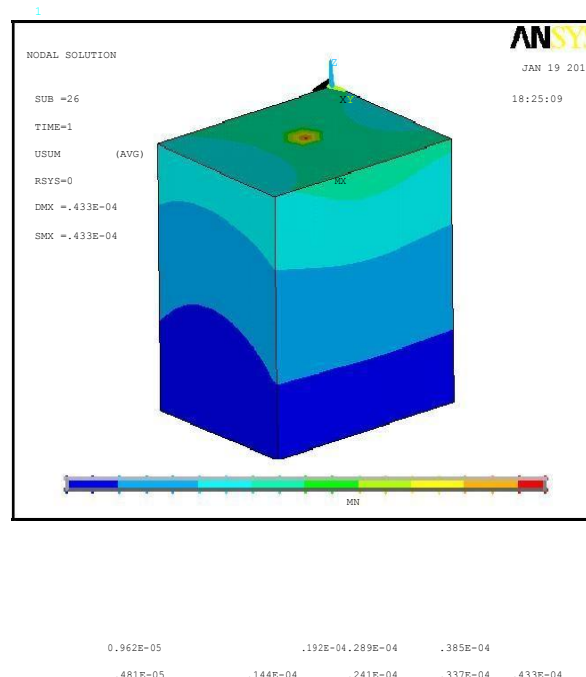
Fig. 8. Deformed foundation under static loading
