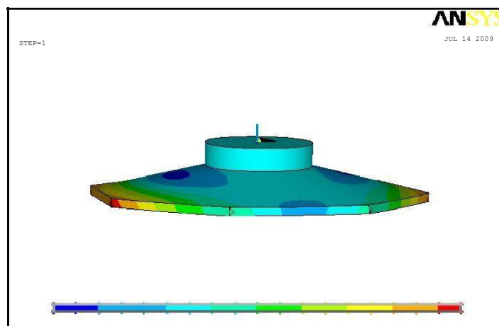
Fig. 12. FE mesh of the octagonal mesh with the column
