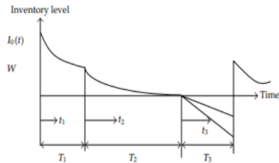
Graphical Representation of the OW inventory system
