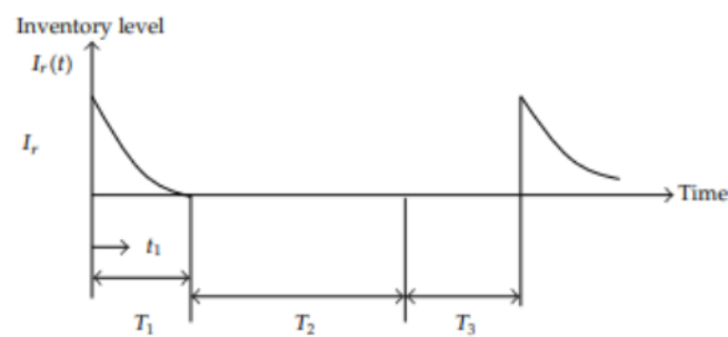
Graphical Representation of the RW inventory system.
