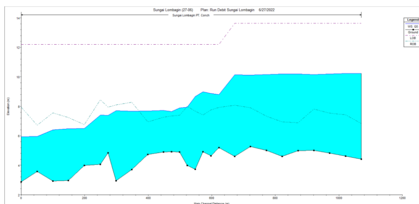
Figure 7. Longitudinal Profile of Lombagin River Channel Against 5-Year Plan Flood Discharge
