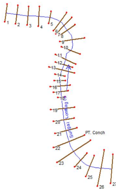
Figure 5. Pipeline Geometry schematization at the review point
