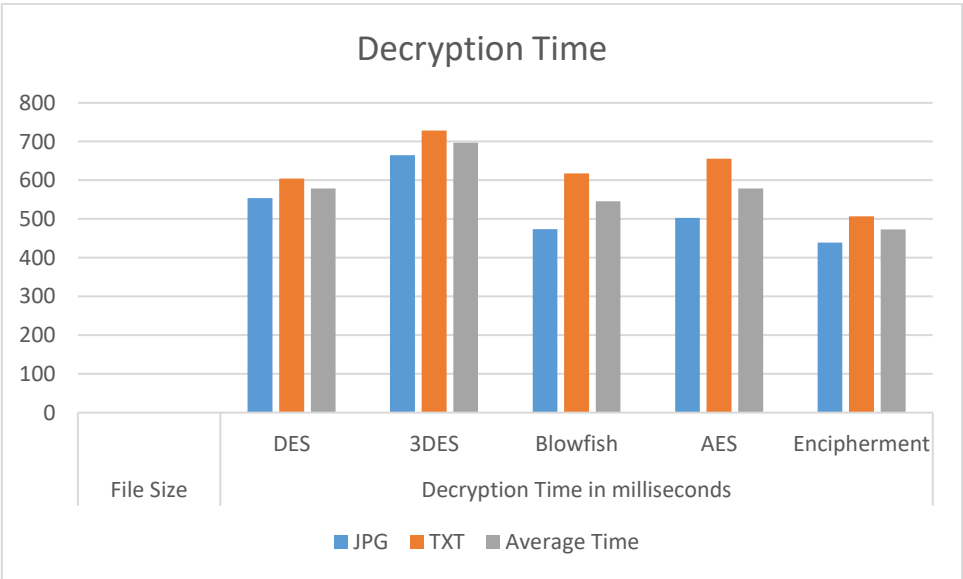
Fig 5.2 Decryption Time
