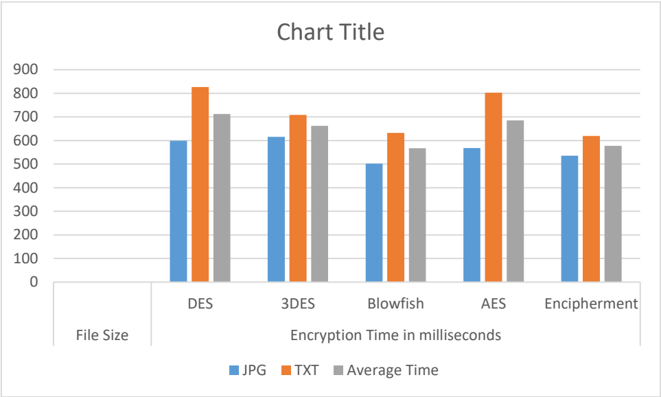
Fig 5.1 Encryption time
