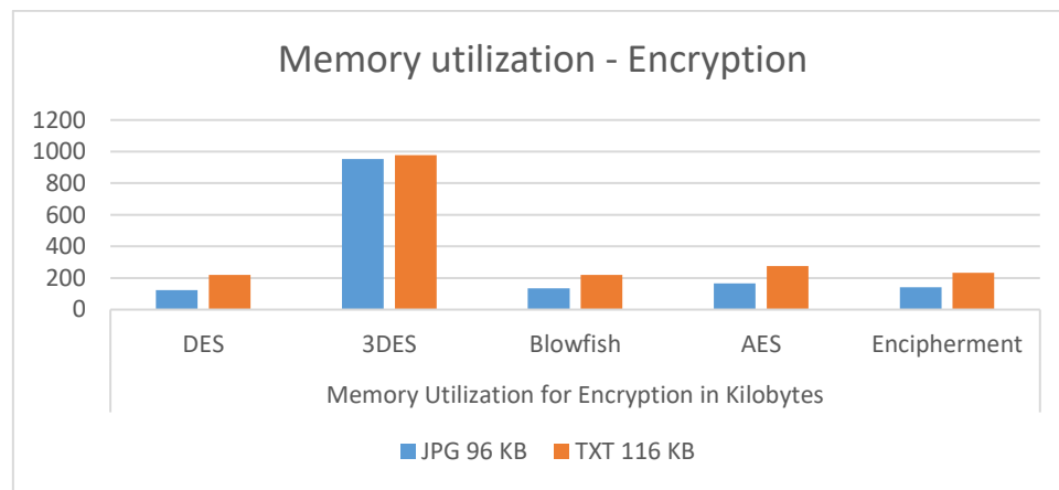
Fig 5.3 Memory utilization for encryption
