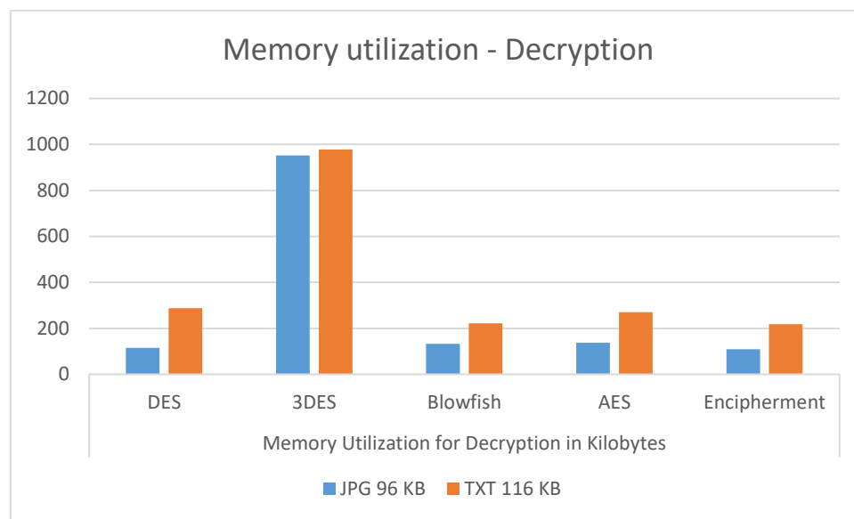
Fig 5.4 Memory Utilization for Decryption
