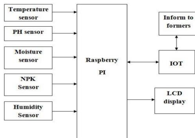
Fig 8: Working model of soil nutrient monitoring.
