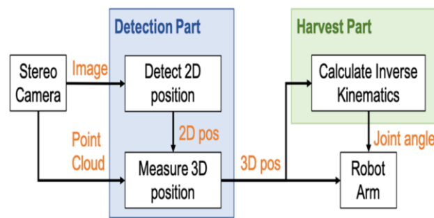
Fig 3: Working of selective harvesting.
