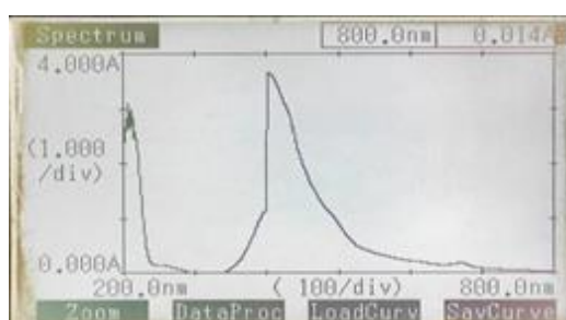
Figure 2. UV-visible absorption spectra of optimized sample of silver nanoparticle (AgNP1).
